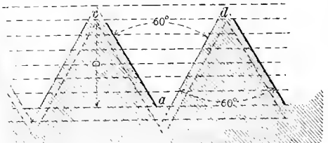
Fig. 4497. SELLERS' STANDARD SCREW-THREADS U. S. and M. C. B. standard.
